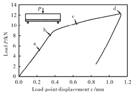
Fig. 5 Load versus load-point displacement curve obtained
