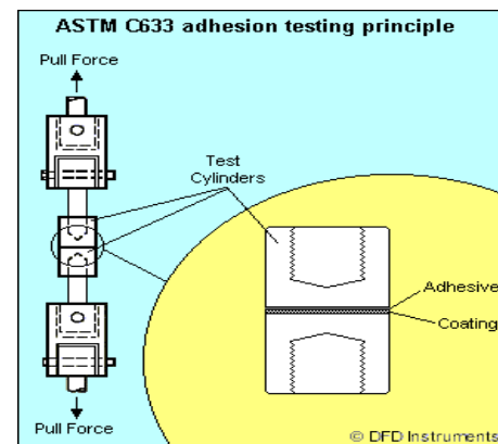
Fig. 2 Tension test of coated sample
